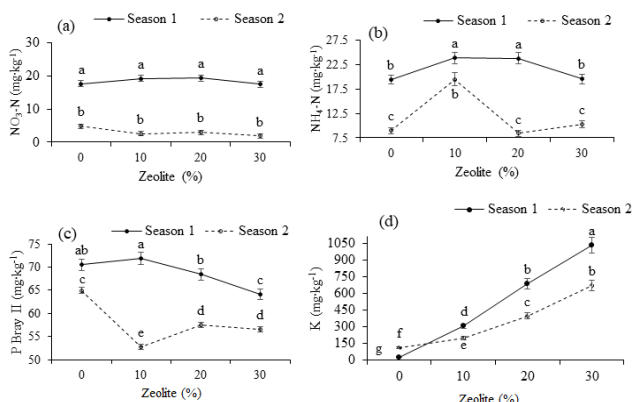
Fig-6 (a-d). Chemical status of cabbage potting soil in response to the applied zeolite. Bars with the same letter are not significantly different, LSD ( P=0.05 ) = (a) 5.04 (b) 3.14 (c) 2.22 (d) 57.49.
