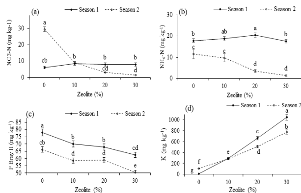
Figure-7 (a-d). Effect of zeolite on the chemical status of Swiss chard potting soils at the end of each season. Bars with the same letter are not significantly different, LSD ( P=0.05 ) = (a) 3.37 (b) 2.57 (c) 4.05 (d) 55.50.
