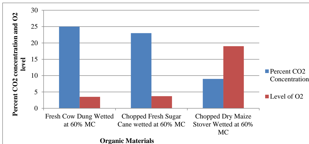
Figure 1. CO 2 and O 2 content of bio-generators obtained by composting organic materials at 60% MC after 48 h period of incubation period
